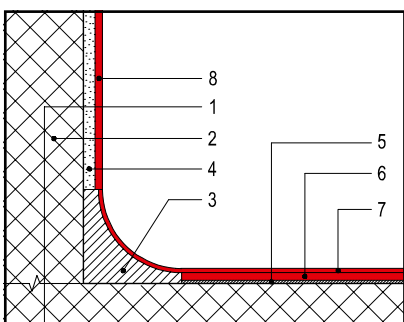
Raccords courbes rigides
